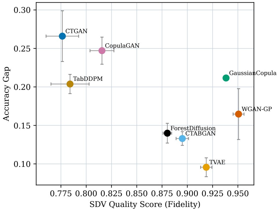
Wine Quality: SDV Quality Score (Fidelity) vs Accuracy Gap
